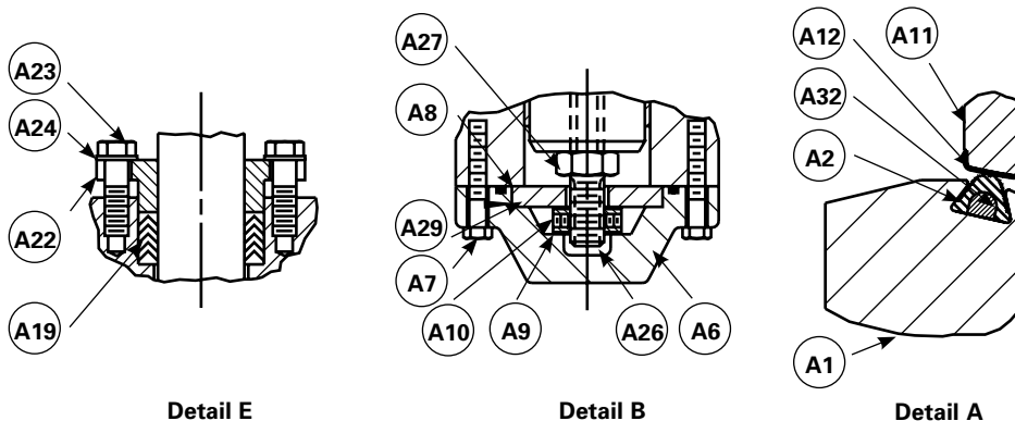
Detail E Adjustable Packing Optional on 24-48" (600-1200mm) Standard on 54-72" (1400-1800mm)
